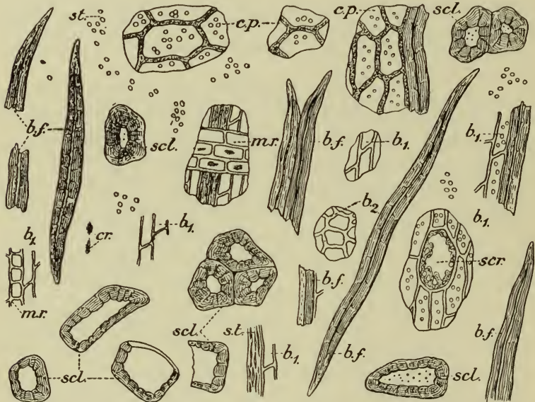
FIG. 97.—Powdered Cinnamon Bark. b_1 , b_2 , bast parenchyma in longitudinal and in transverse section ; b.f. , bast fibres ; c.p. , cortical parenchyma ; cr. , crystals of calcium oxalate ; m.r. , medullary ray ; s.t. , collapsed sieve tissue ; scl. , sclerenchymatous cells ; scr. , secretion cells ; st. , starch. (Partly after Greenish and Collin.) \times 150 .
